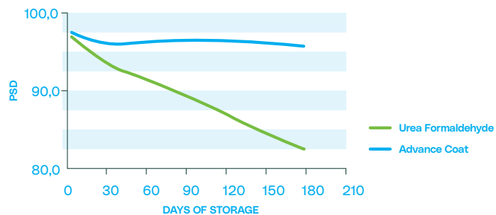
Granulometry 2.5 - 1.0 mm
